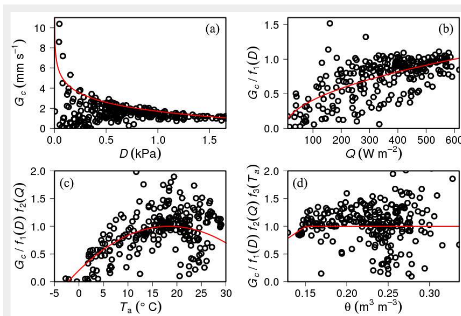
Fig. 2 - Relationships (a) between vapor pressure deficit ( D ) and canopy conductance ( G_c ), (b) between photosynthetic active radiation ( Q ) and G_c divided by estimated G_c using D only ( f_1(D) ), (c) between air temperature ( T_a ) and G_c divided by estimated G_c by using D and Q ( f_1(D)f_2(Q) ), and (d) between volumetric soil water content ( \theta ) and G_c divided by estimated G_c by using D , Q , and T_a ( f_1(D)f_2(Q)f_3(T_a) ). The red line in each plot indicates the function expressing the response of G_c to D , Q , T_a , and \theta , respectively. The data from single plot and single growing season were shown.
